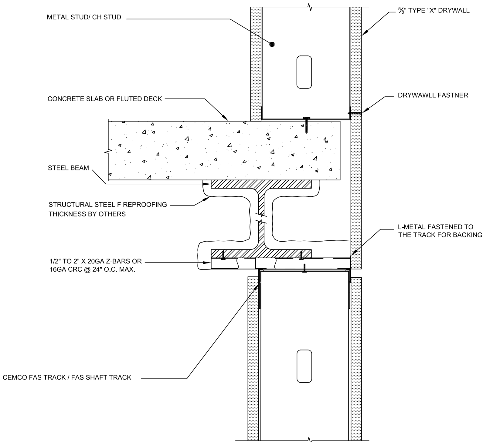
HW-D-0551 STAIRWELL SLAB BY PASS @ I- BEAM
