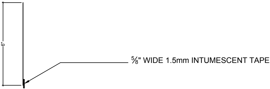
CEMCO FAS-RBR STRAP (RECESSED BASE REVEAL)
